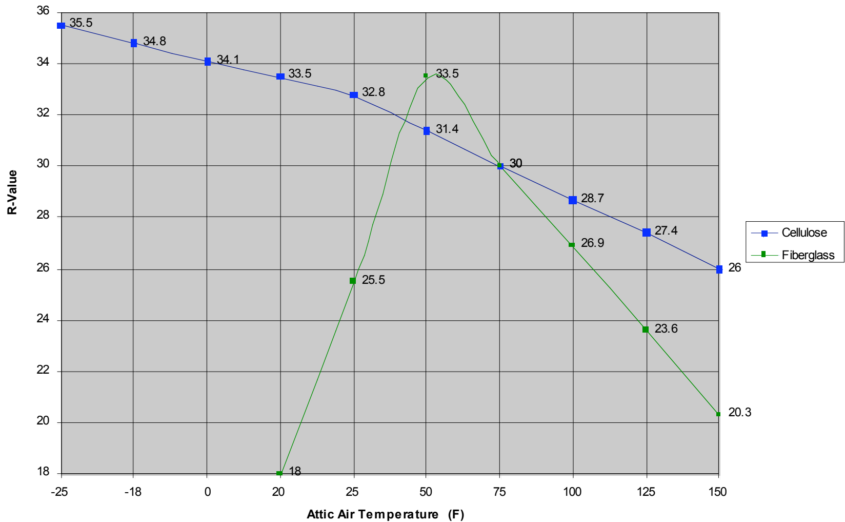
Attic Temperature vs. R-Value (Fiberglass & Cellulose)
